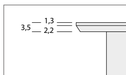
PROFILO PIANO LEGNO WOODEN TOP PROFILE
