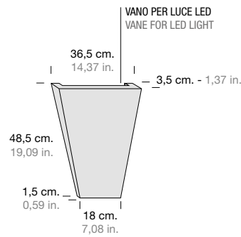
FORMELLA IN LEGNO "A" E "B" "A" AND "B" WOODEN TILE
