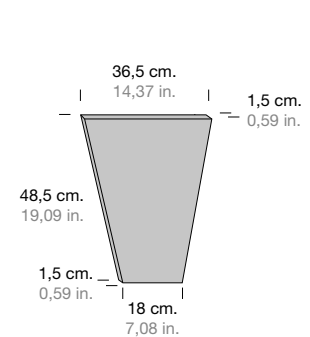
FORMELLA C TILE C
