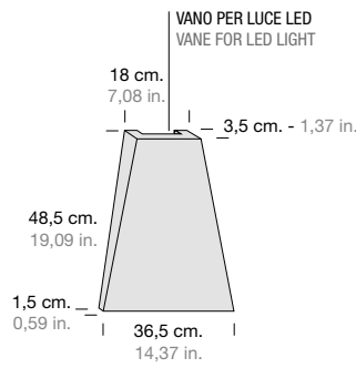
FORMELLA B TILE B
